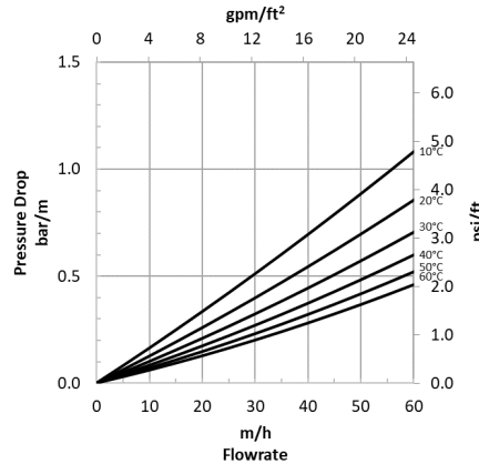
Figure 1: Pressure Drop
